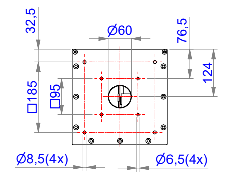
Standard bottom plate
