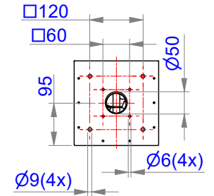
Standard bottom plate
