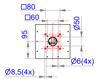
Bottom plate for MCVi-1
